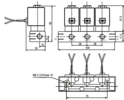
1 IN 3 OUT 2/2 WAY DIRECT ACTING SOLENOID VALVE WITH 1/8" SCREWED FEMALE CONNECTION
