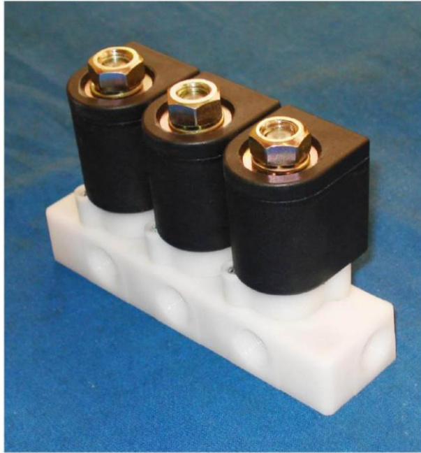
1 IN 3 OUT 2/2 WAY DIRECT ACTING SOLENOID VALVE WITH 1/8" SCREWED FEMALE CONNECTION
