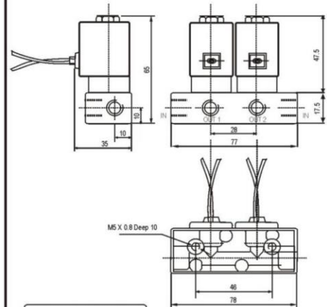
1 IN 2 OUT 2/2 WAY DIRECT ACTING SOLENOID VALVE WITH 1/8" SCREWED FEMALE CONNECTION
